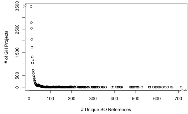
Fig. 1: Number of SO references in GitHub projects.
