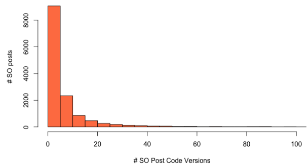
Fig. 7: Evolution of code snippets in SO posts.
