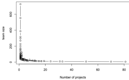
Fig. 2: GitHub team size distribution.
